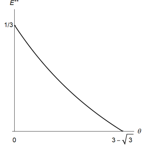
Figure 3. Graph of the total concentrations, E^{**}(\theta)
