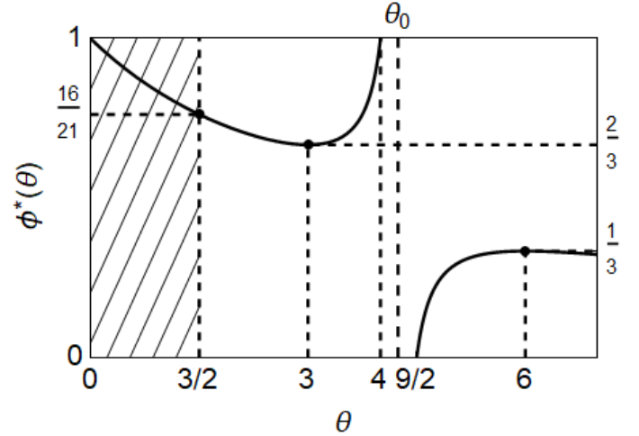
Figure 2. Optimal abatement technology, \phi^*(\theta)
