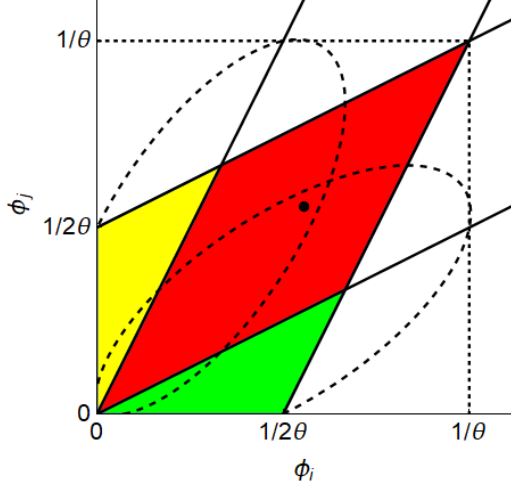
Figure 1. Feasible region of \phi_i and \phi_j
