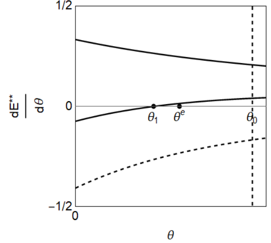
Figure 4. Effects on the total concentrations
